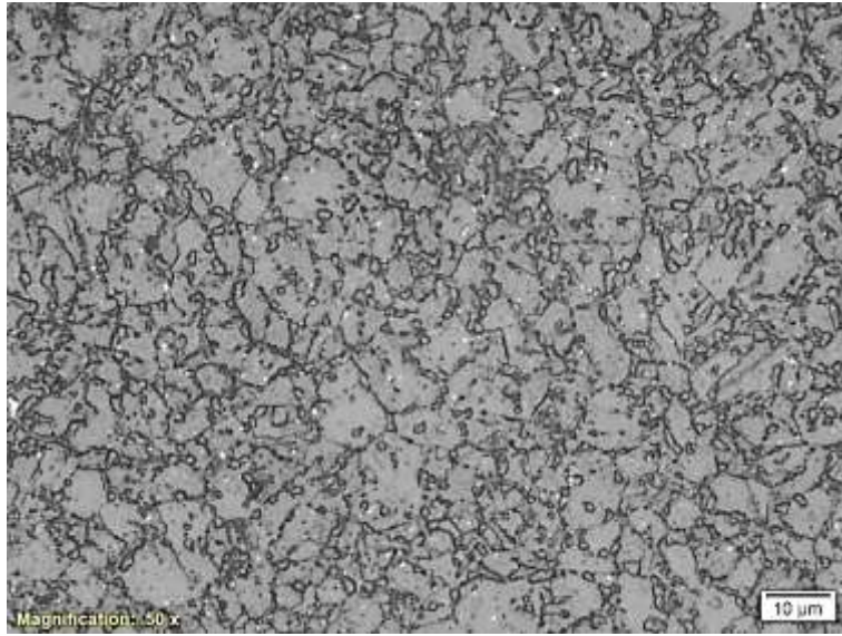
Case 1 T91 (nital 9%)
