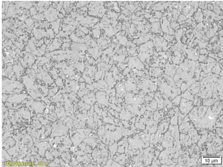
Case 2 T91 (nital 9%)
